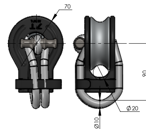
Poulie LB 7T MWL Ref: Poids / Weight : 461g
