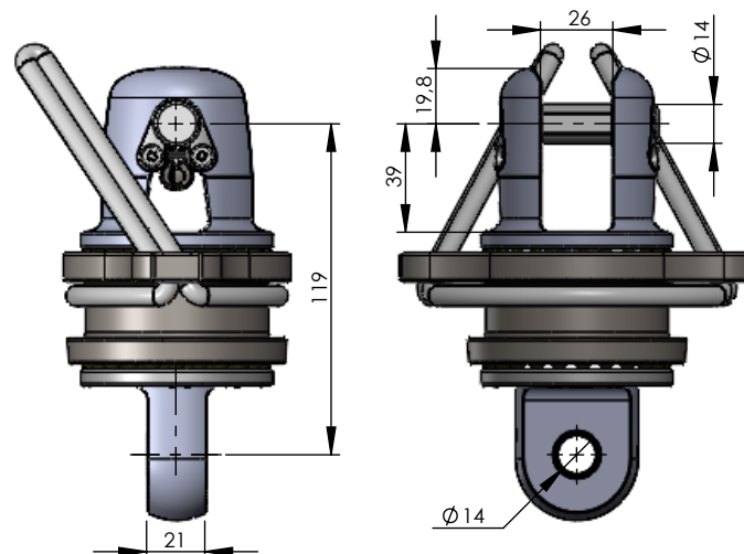
cosse fast 7000 / Fast Thimble Ref: Poids / Weight : 1170g
